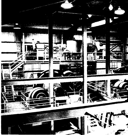
Machinery for pulverizing ore.
